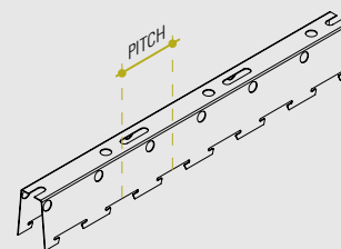
Carrier TR9
