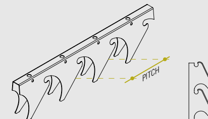
Carrier TR7 - 30°
