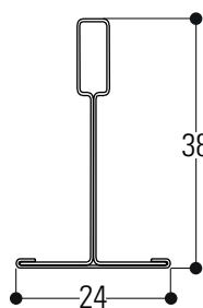
Section: PP 3700 mm
