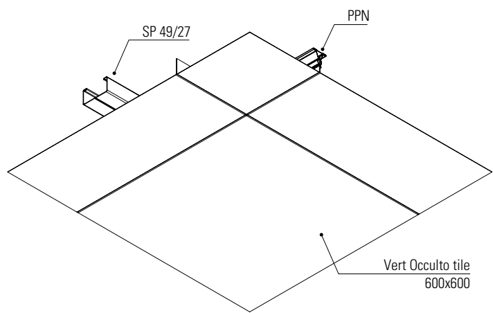
VIEW FROM BELOW Double frame with SP 49/27
