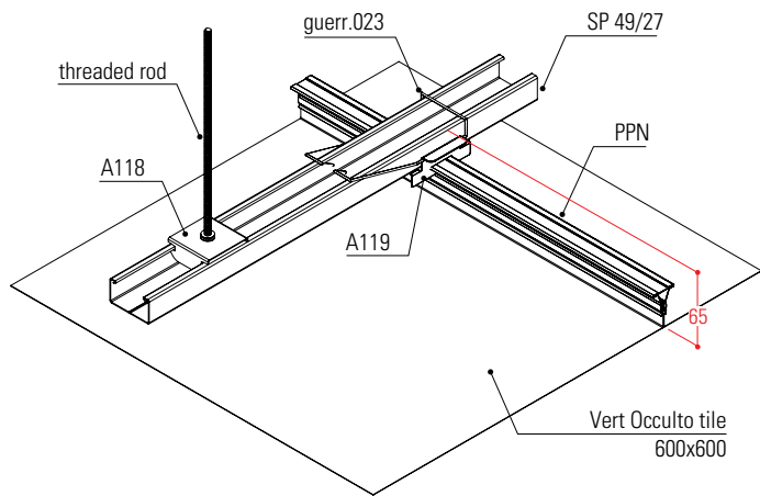
VIEW FROM ABOVE Double frame with SP 49/27
