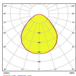
Vert Reticula Led 100 32W UGR
