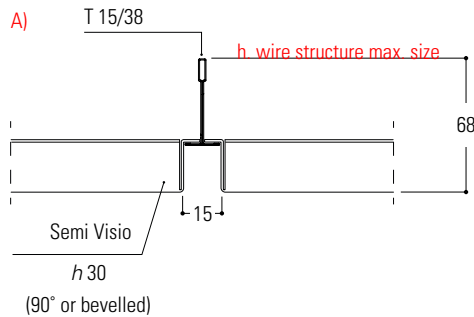
System with plenum
