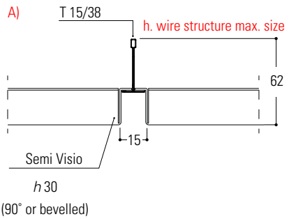
System with plenum
