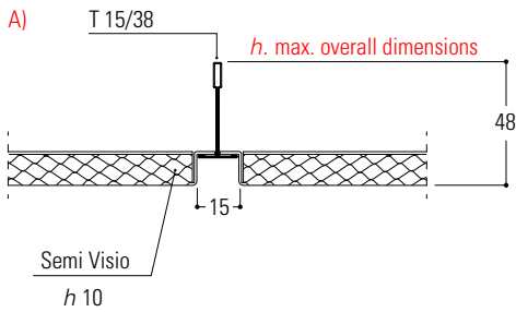
System with plenum
